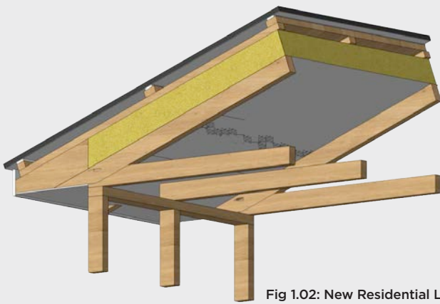
Fig 1.02: New Residential Longrun roofing - Trussed or Skillion
